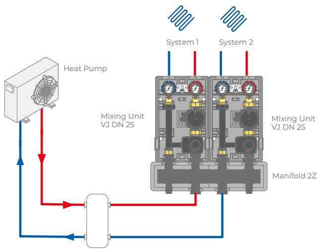
Example of system with ZZ collector and water taken from technical storage tank
