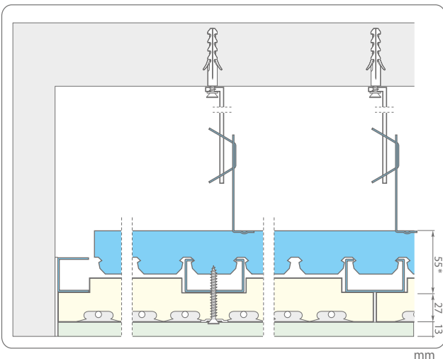
Hanging structure with snap profile
