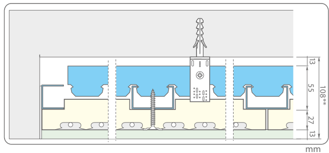
Structure with snap profile
