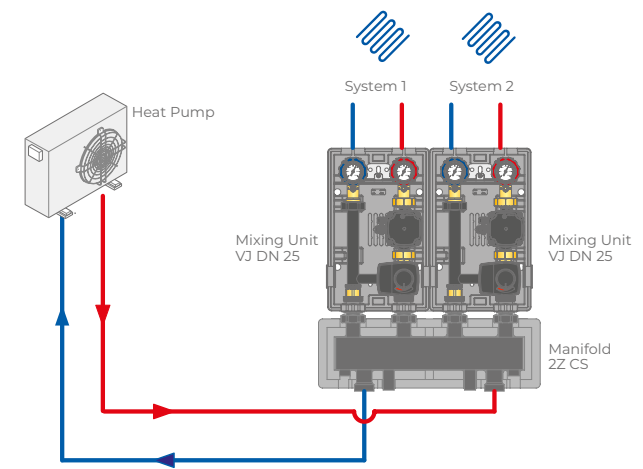
System example with ZZ-CS manifold and water directly supplied from heat pump
