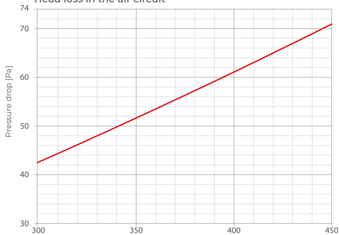
Head loss in the air circuit
