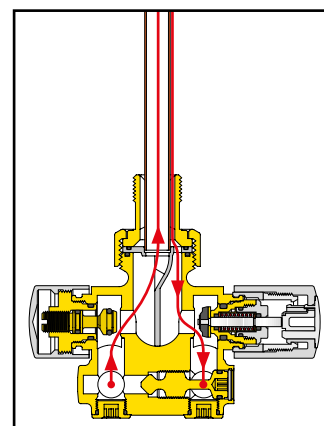
Application bitube
