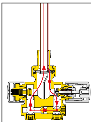
Application monotube
