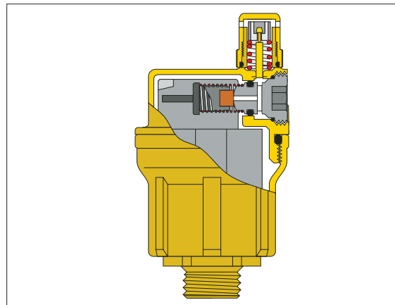
Construction detail for NA5026 PLUMBVENT™
