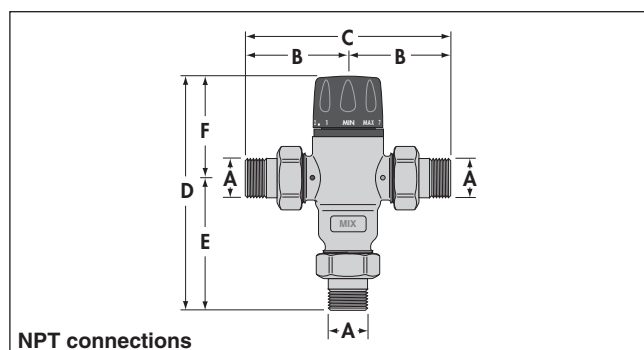
NPT connections
