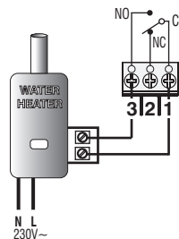
Connection to a water heater
