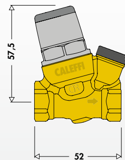
Micro pressure reducing valve 3/8"
