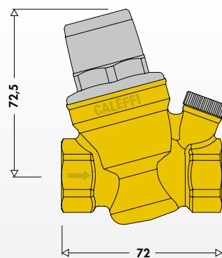
Standard pressure reducing valve 1/2"
