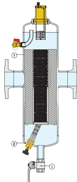
Steel DISCALDIRTMAG NA546_M series
