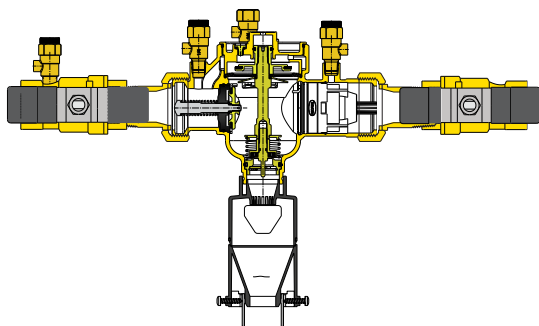
1 1/2 inch model
