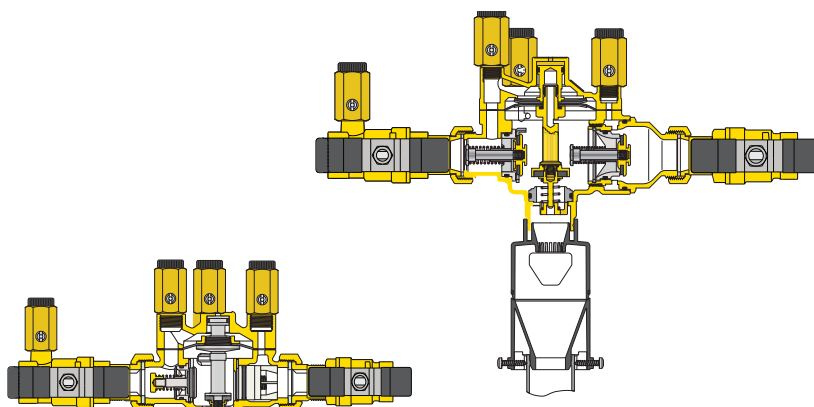
3/4 & 1 inch model
