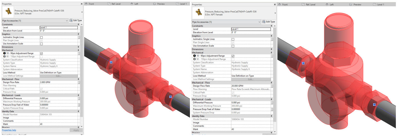
Figure 5 – The Caleffi PresCal HP Heavy-duty Piston-type 536A Series Pressure Reducing Valve family can be found under pipe accessories in the project browser and placed directly onto pipe of the same size. It will then read flows and consider pressure drop in the system. In the figure, a flow warning is shown when flow through the accessory exceeds the maximum allowable.
