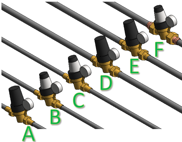
Figure 3 - Caleffi 535H PresCal Pressure Reducing Valve
