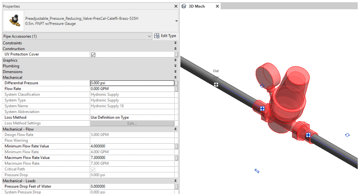
Figure 5 – The Caleffi 535H PresCal Pressure Reducing Valve family can be found under pipe accessories in the project browser and placed directly onto pipe of the same size. It will then read flows and consider pressure drop in the system. Options such as selecting the visibility of a UV Protection Cover are available.
