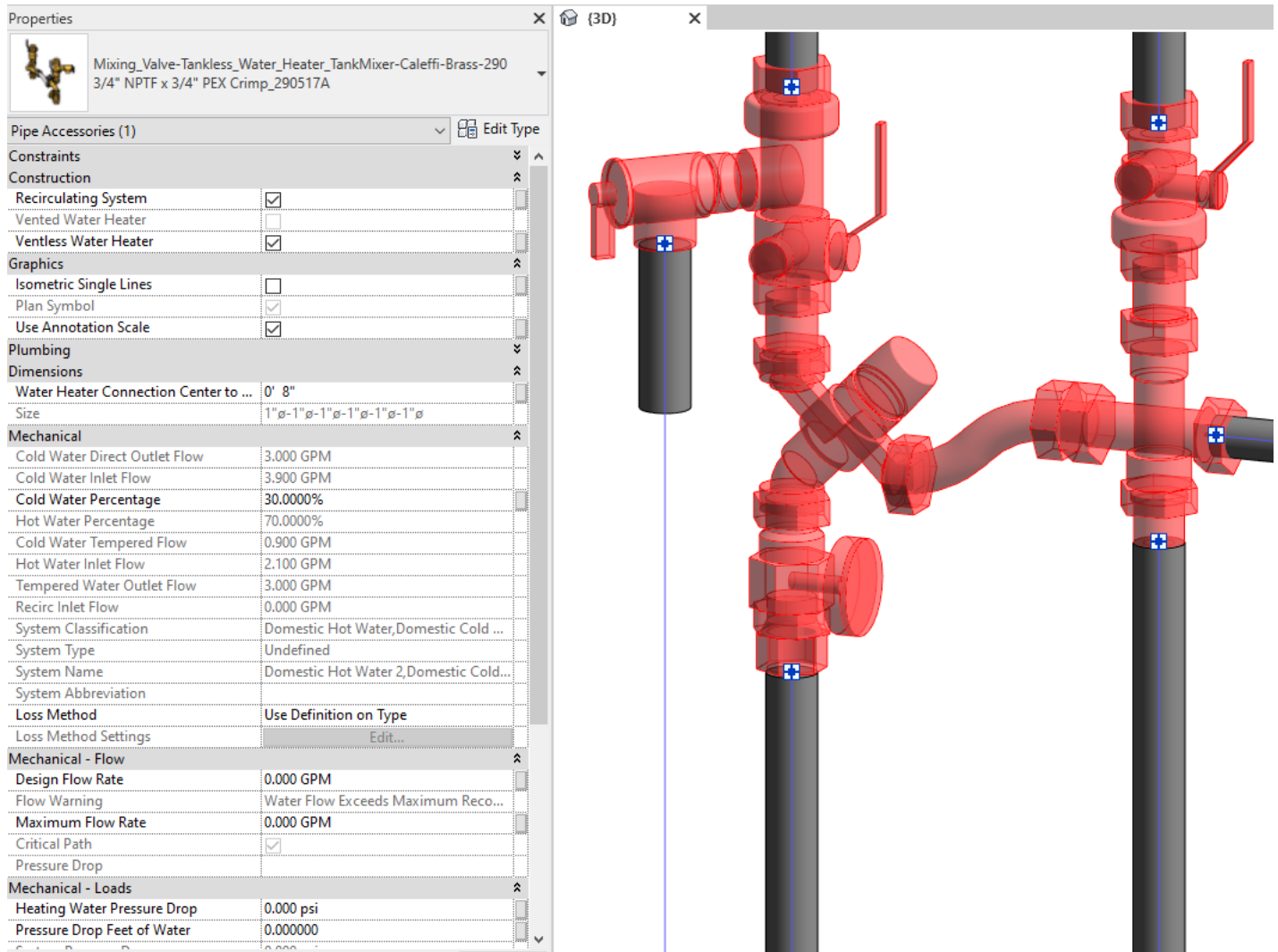
Figure 5 – The Caleffi 290 Series Tankless Water Heater Service Valve Kit with 520 Series Tankmixer and Tankless Water Heater Service Valve Kit families can be found under pipe accessories in the project browser and placed directly onto pipe of the same size. It will then read flows and consider pressure drop in the system.
